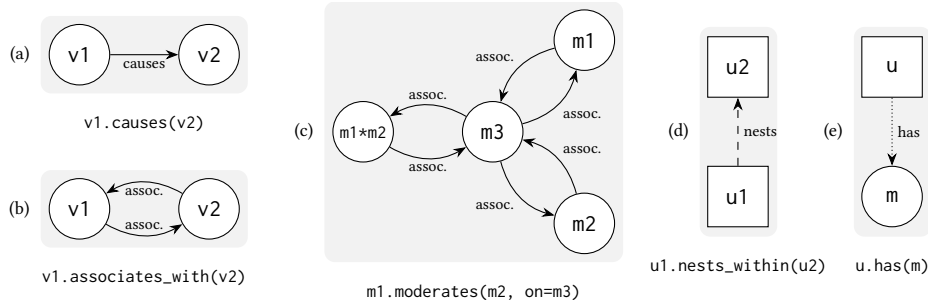
Figure 5.2: Code snippets of conceptual and data measurement relationships written in Tisane’s DSL and their representation in Tisane’s graph IR.
