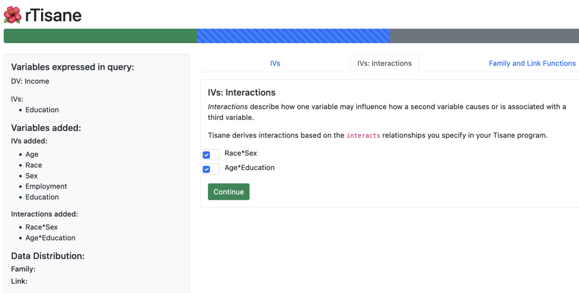
Figure 6.2: rTisane’s statistical model disambiguation interface.
