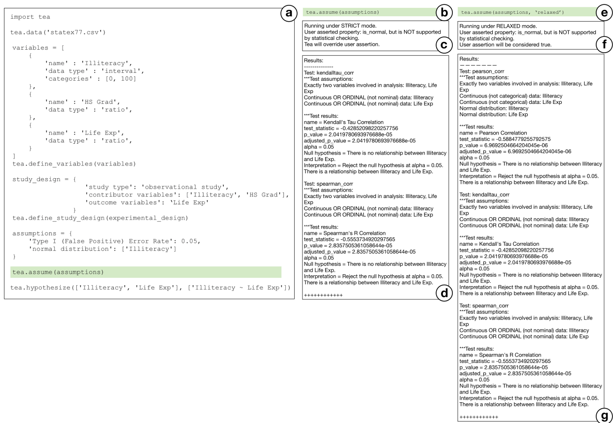
Figure 3.1: Tea program and its mode-dependent executions.
