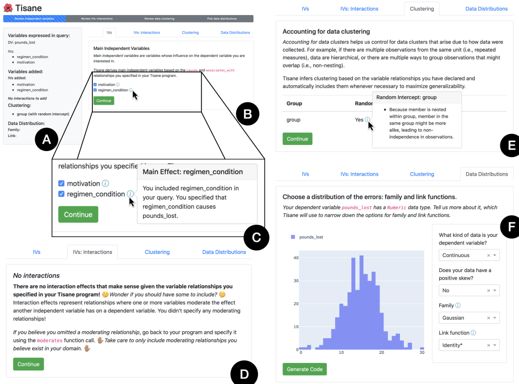
Figure 5.4: Example Tisane GUI for disambiguation.
